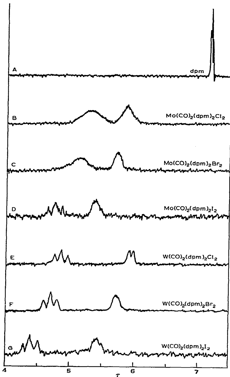
Fig. 1. NMR spectra of \text{M(CO)}_2(\text{dpm})_2\text{X}_2 (methylene proton region); A, dpm; B, \text{Mo(CO)}_2(\text{dpm})_2\text{Cl}_2 ; C, \text{Mo(CO)}_2(\text{dpm})_2\text{Br}_2 ; D, \text{Mo(CO)}_2(\text{dpm})_2\text{I}_2 ; E, \text{W(CO)}_2(\text{dpm})_2\text{Cl}_2 ; F, \text{W(CO)}_2(\text{dpm})_2\text{Br}_2 ; G, \text{W(CO)}_2(\text{dpm})_2\text{I}_2 .
